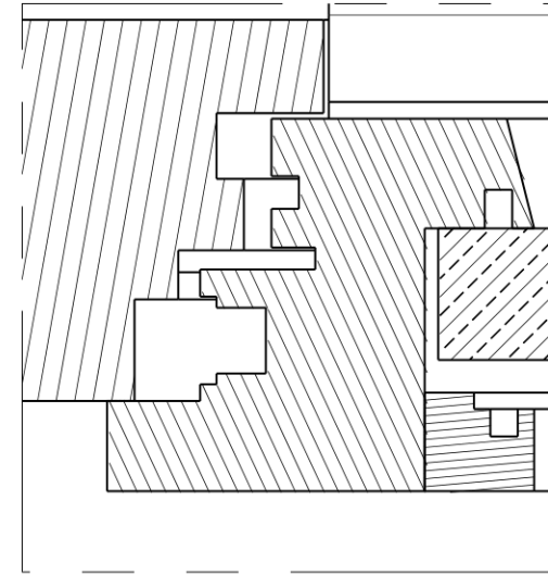
Detail B
